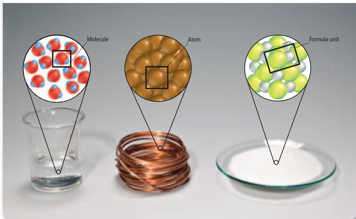
■ Figure 10.2 The amount of each substance shown is 6.02 \times 10^{23} or 1 mol of representative particles. The representative particle for each substance is shown in a box. Refer to Table R-1 on page 968 for a key to atom color conventions.
